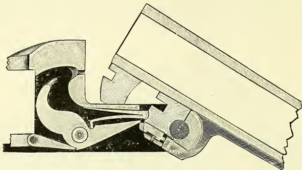
Mechanism of Greener's Patent Hammerless Lock.
